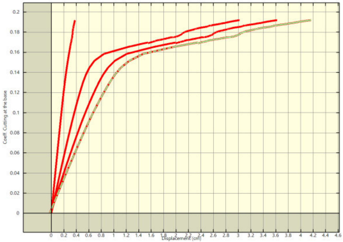
Pushover analysis "Pushover -X Acc" : capacity curve.
