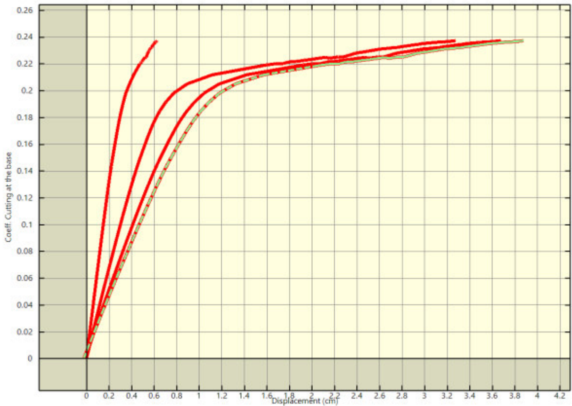
Pushover analysis "Pushover -X Massa" : capacity curve.
